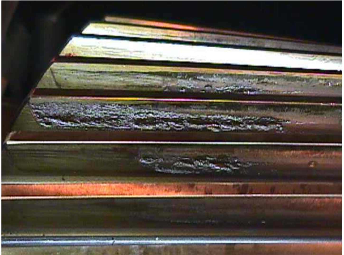
Failure by Loss of Lubrication
